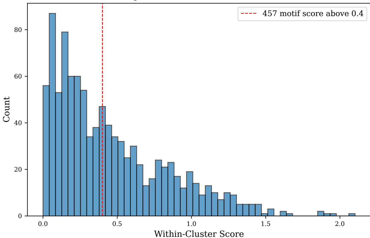
Distribution of All Motif Scores Downsampled to R=100 (50 seeds, 999 motifs total) sigma=(0.02, 0.4), vol=(0.07, 0.9)
